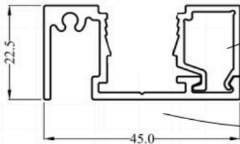
Dolo 45.02, 03
